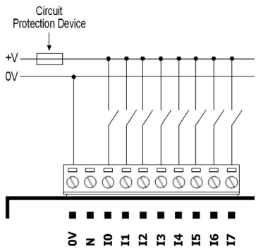
pnp (source) digital input wiring
