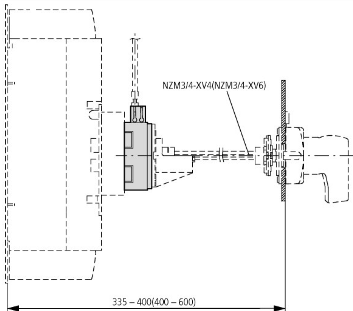
NZM4-XMV + NZM4-XTVD(V)(R)
