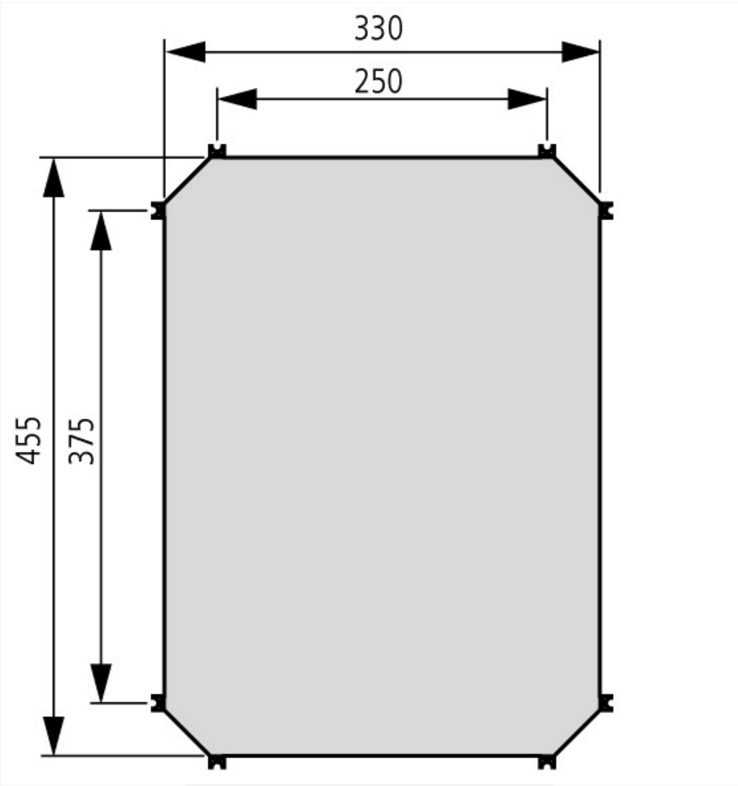
Mounting plate M3-....: 3 mm thick
