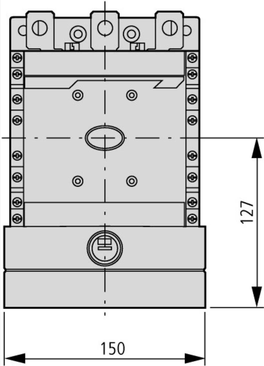
Contactor with star-point bridge and terminal shroud for DILM185A to DILM300A
