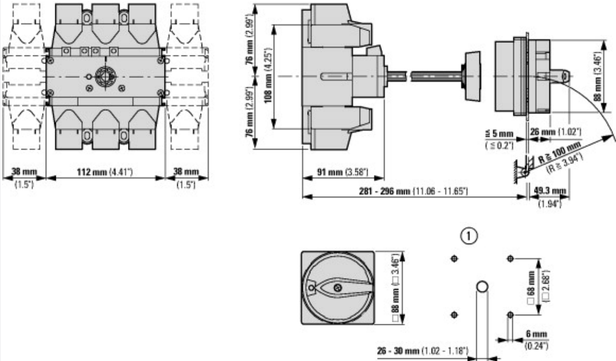
① Drilling dimensions door Distance from mounting plate to front with complete axis.
