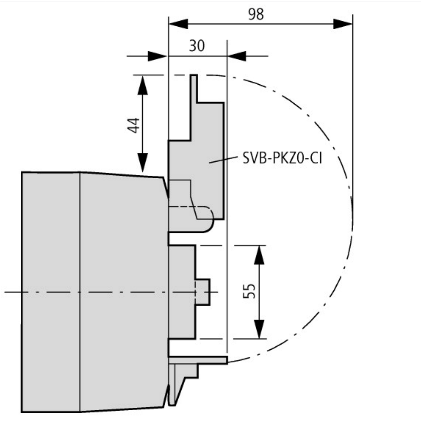
Insulated enclosure for top mounting
