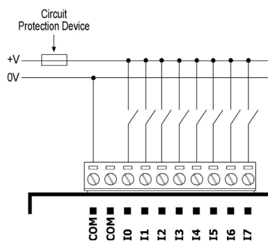
pnp (source) high-speed counter
