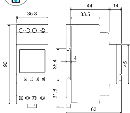
12.31 Screw terminal
