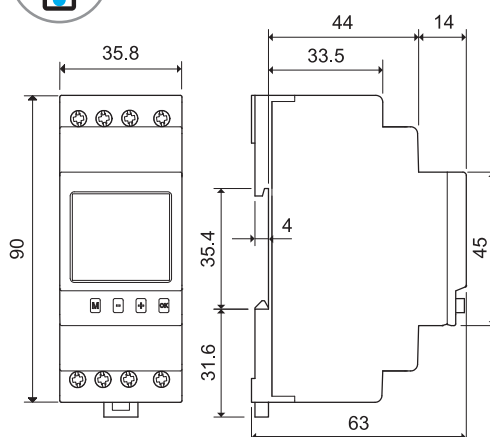
12.51/12.81 Screw terminal
