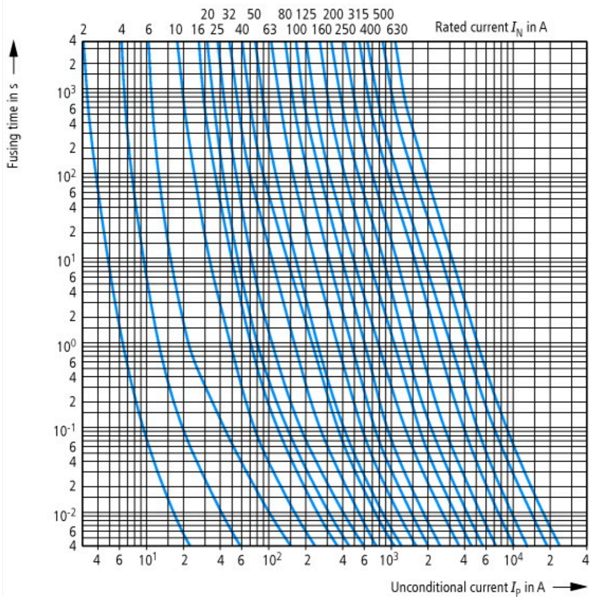
Time-current characteristic
