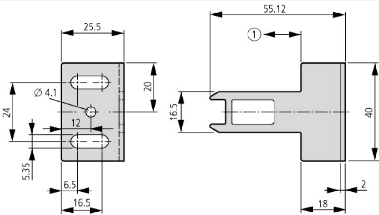
pin with a 4 mm pin after mounting ① Distance to device head = 0.1 ... 3.0 mm
