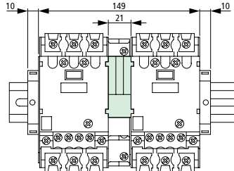
Mechanical interlock for high-capacity contactor modules MV-PKZ2
