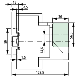
Mechanical interlock for high-capacity contactor modules MV-PKZ2
