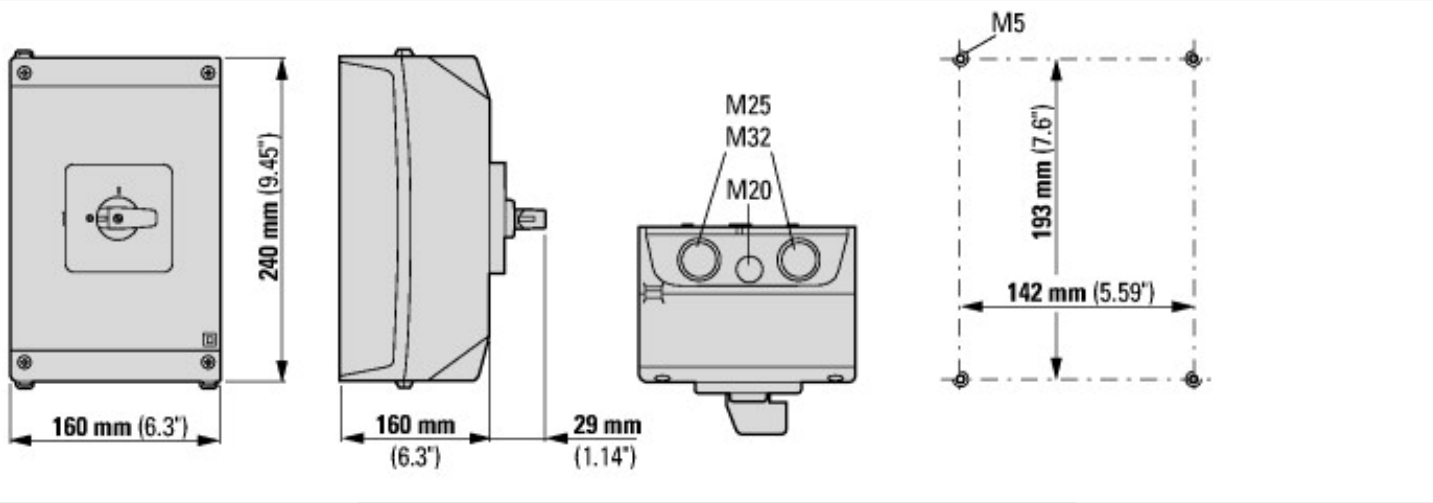
Cam switches T5B and T5 are of identical design, only their contacts are different
