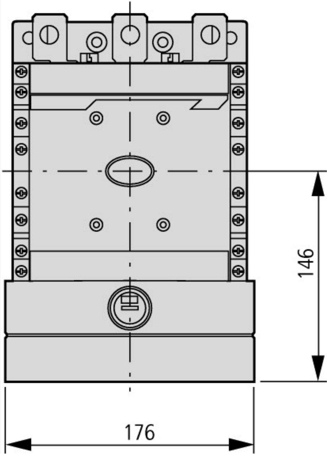
Contactor with star-point bridge and terminal shroud for DILM500
