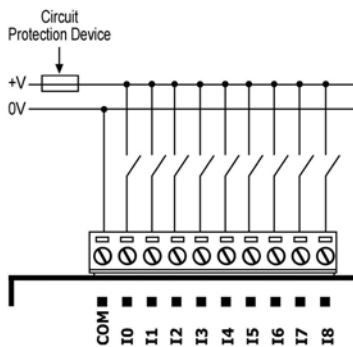
pnp (source) digital input wiring
