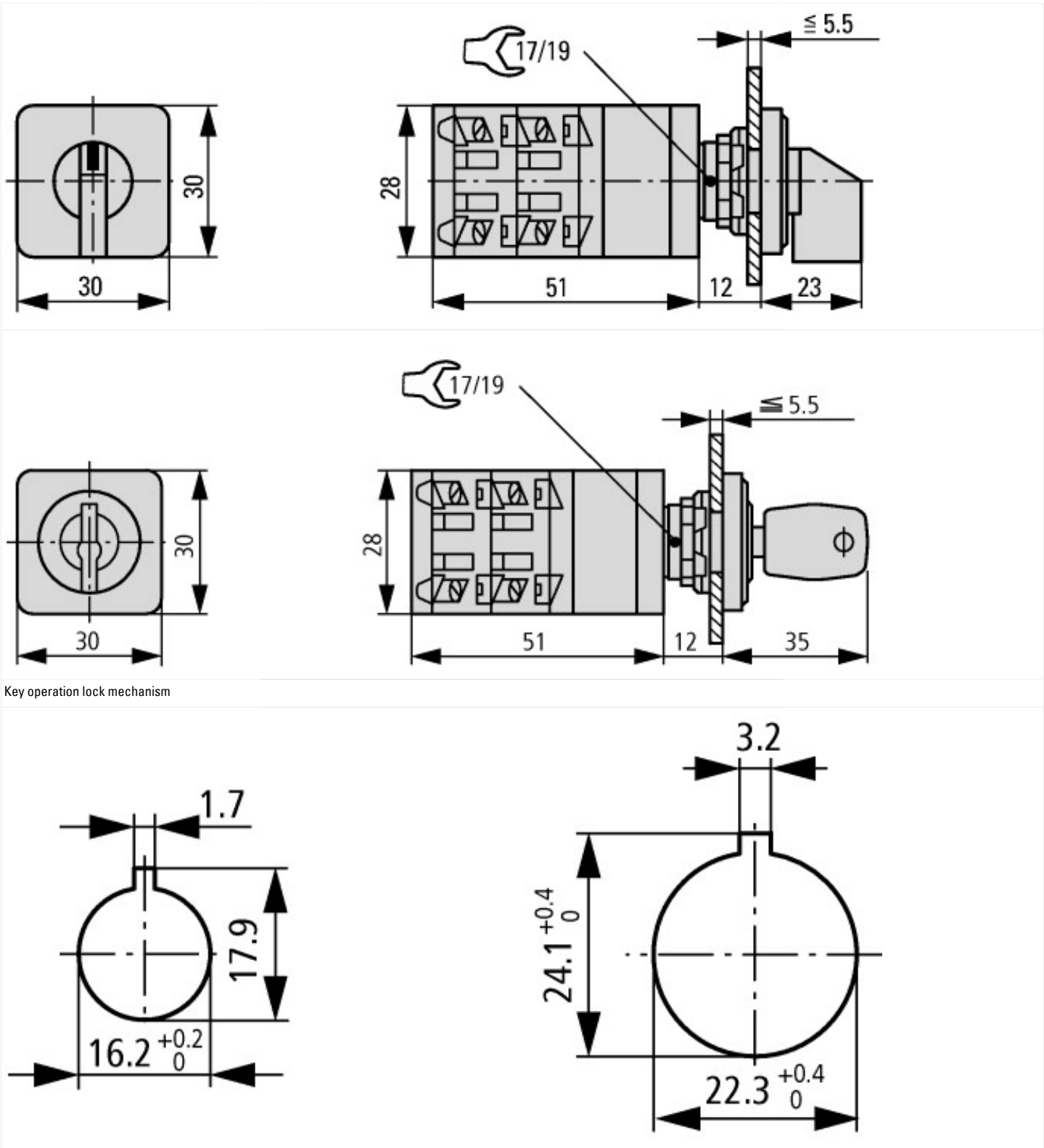
Door drilling dimensions Drilling dimensions: either 16.2 mm = without reduction \triangle RMQ16 or 22.3 mm = with reduction \triangle RMQ Titan
