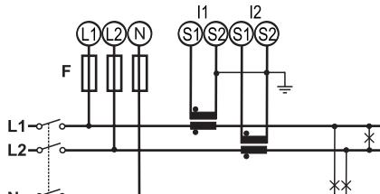
Fig. 15 Two-phase system (3-wire), 2 CT. 315 mA fuse (F).
