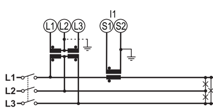
Fig. 14 Three-phase system without neutral (3-wire), balanced load, 1 CT and 2 VT/PT.
