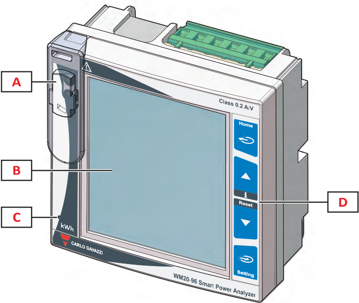
Fig. 1 Front
