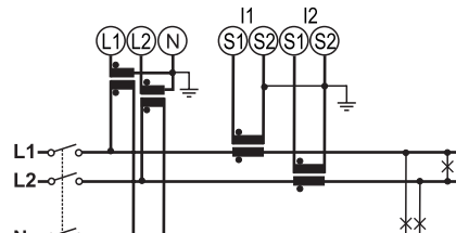
Fig. 16 Two-phase system (3-wire), 2 CT and 2 VT/PT.
